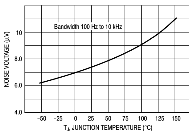
Figure 15. Output Noise
