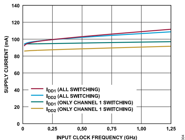
Figure 8. Supply Current vs. Input Clock Frequency for the ADN4622
