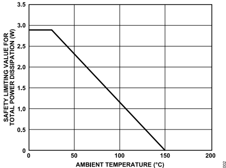
Figure 3. Thermal Derating Curve, Dependence of Safety Limiting Values with Ambient Temperature per DIN V VDE V 0884-11, SOIC_W_FP
